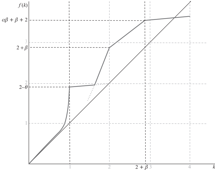
Figure 1 The function f^\epsilon defined in Equation (4).
